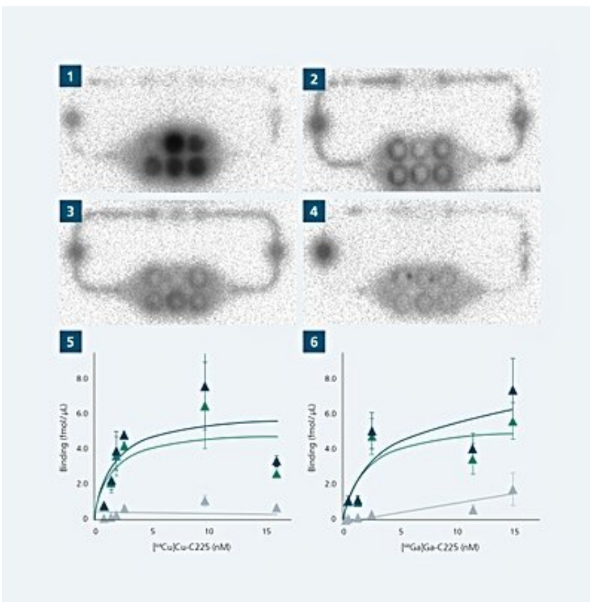
Binding of [^{68}\text{Ga}]\text{Ga-C225} (2 nM) in MPS-modules on A431 (A) and MDA-MB435S (C); (B) shows the nonspecific binding on A431, (D) on MDA-MB435S (0.8 \mu\text{M} C225); below: graphs of saturation assays on A431 monolayer
