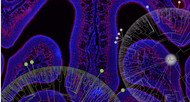
Olfactory signatures corresponding to specific odorants. In the background, an olfactory sensory neuroepithelium. Credit: © Ivan Rodriguez
