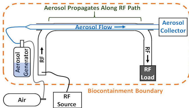
Conceptual schematic showing key portions of the viral aerosol microwave inactivation experiment. Credit: Air Force Research Laboratory.
