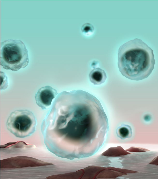
An illustration of natural killer cells. Credit: Val Altounian / AAAS
