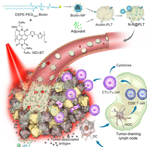
Schematic illustration of the platelet-based formulation and anticancer application in photothermal-immunological combined therapy. Credit: WEI Wei
