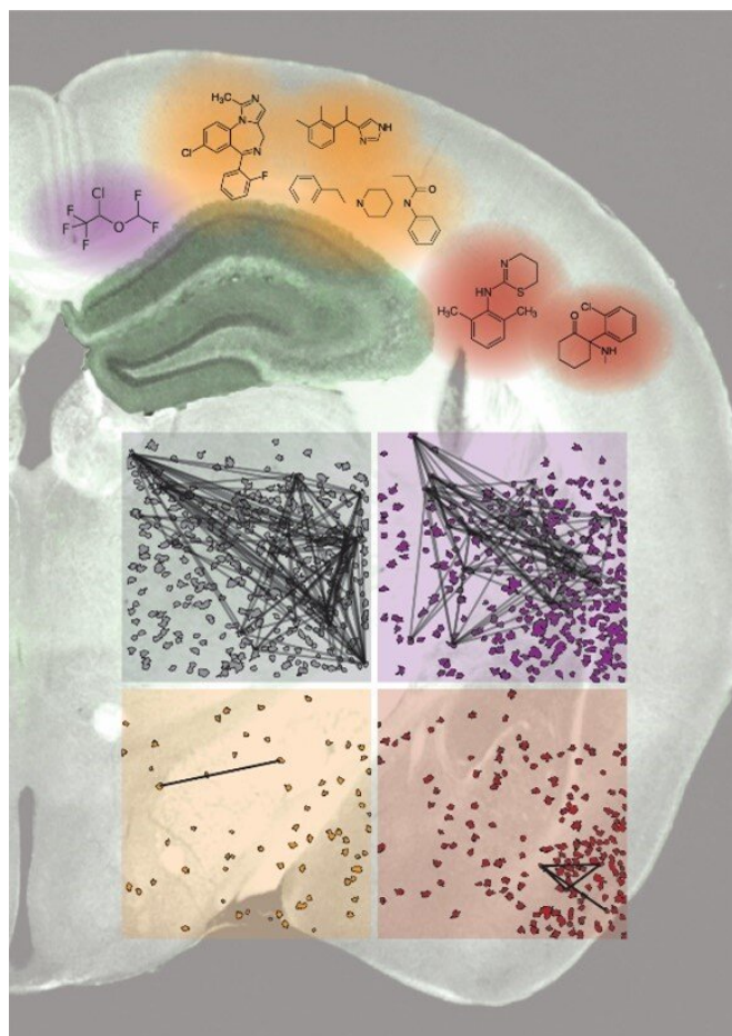
A mouse brain section highlighting the hippocampus is overlaid with the molecular structures of the anesthetics isoflurane (purple), medetomidine/midazolam/fentanyl (orange), and ketamine/xylazine (red). The four panels in the lower part show two-dimensional maps of active neurons in the same hippocampal region during wakefulness (top left) and under the different anesthetics indicated above. Colors indicate the respective anesthetics. Neurons with correlated activity are connected by black lines. Credit: Simon Wiegert, CC-BY
